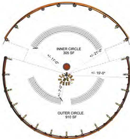
FLOOR PLAN
